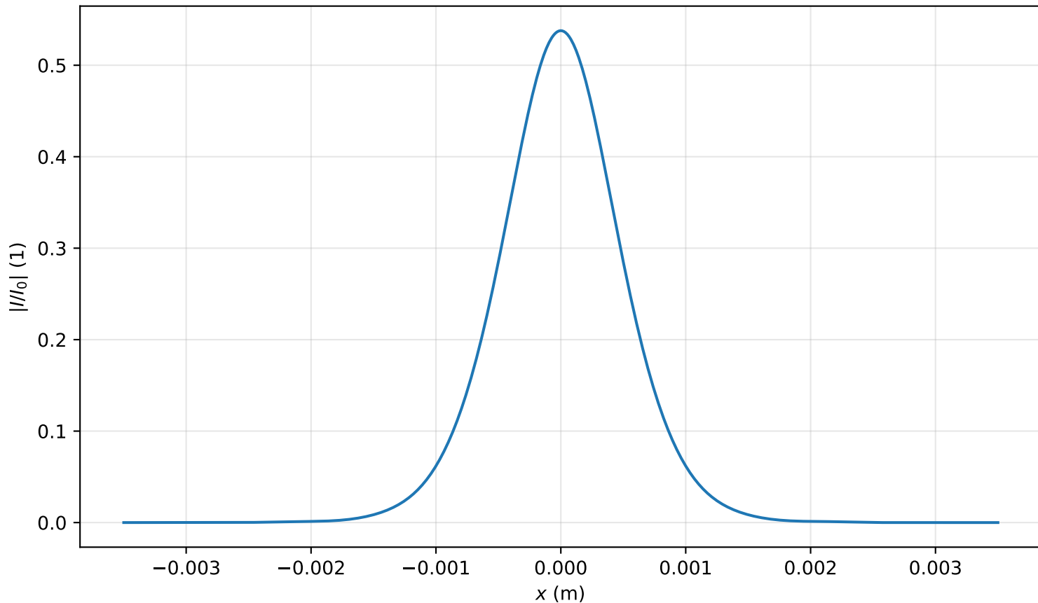
Intensity profile I(x, y = 0, z = 3.662m)/I_0 , P_{in}=0.6P_{cr} , artificial time
